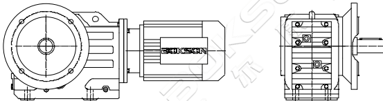
KF...Y.. 法兰轴伸式安装螺旋锥齿轮减速机 Flange-mounted helical-bevel gear units with solid shaft
