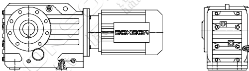
KA...Y.. 空心轴安装螺旋锥齿轮减速机 Helical-bevel gear units with hollow shaft
