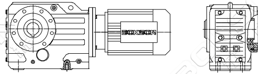
KAZ...Y.. 小法兰空心轴安装螺旋锥齿轮减速机 Short-flange-mounted helical-bevel gear units with hollow shaft
