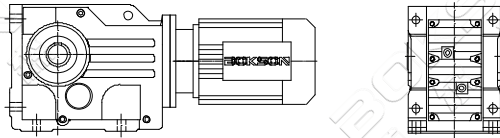
KAB...Y.. 底脚空心轴安装螺旋锥齿轮减速机 Foot-mounted helical-bevel gear units with hollow shaft
