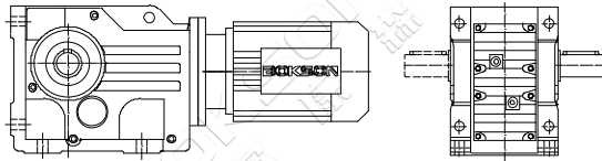
K..Y.. 底脚轴伸式安装螺旋锥齿轮减速机 Foot-mounted helical-bevel gear units with solid shaft
