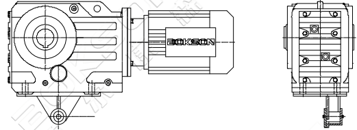
KAT...Y.. 带防转臂空心轴安装螺旋锥齿轮减速机 Torque-arm-mounted helical-bevel gear units with hollow shaft
