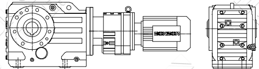
KA (K, KF, KAF, KAB, KAZ) ...R...Y... 组合式螺旋锥齿轮减速机 Combinatorial helical-bevel gear units
