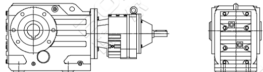
KA (K, KF, KAF, KAB, KAZ) S...R... 轴输入的组合式螺旋锥齿轮减速机 Shaft input combinatorial helical-bevel gear units
