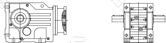
KA (K, KF, KAF, KAB, KAZ) ...Y... 电机用户自配或配特殊电机时需加联接法兰 When equipping the user's motor or the special one, the flange is required to be connected
