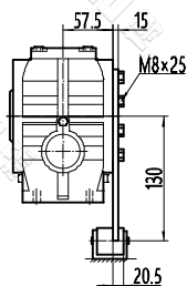
SAT47
