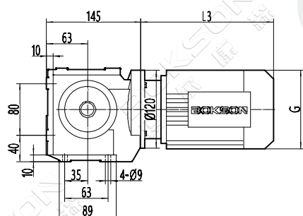
S37
