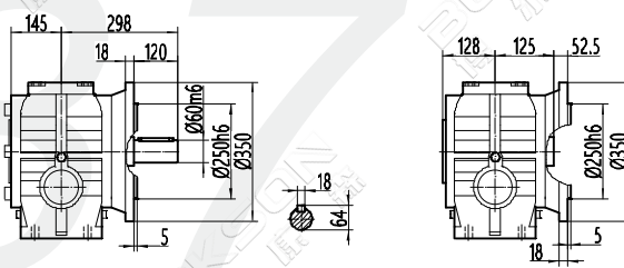
SAF87
