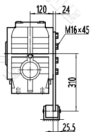
SAT87
