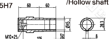
SA47/SAZ47/SAF47空心轴
